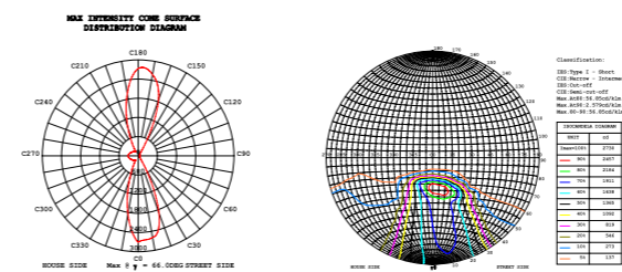
30W Solar LED Street Light IES
