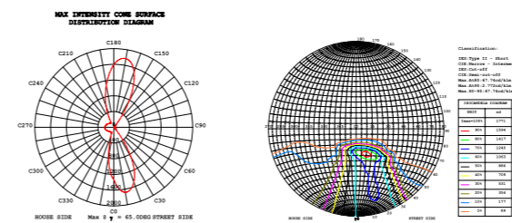
20W Solar LED Street Light IES
